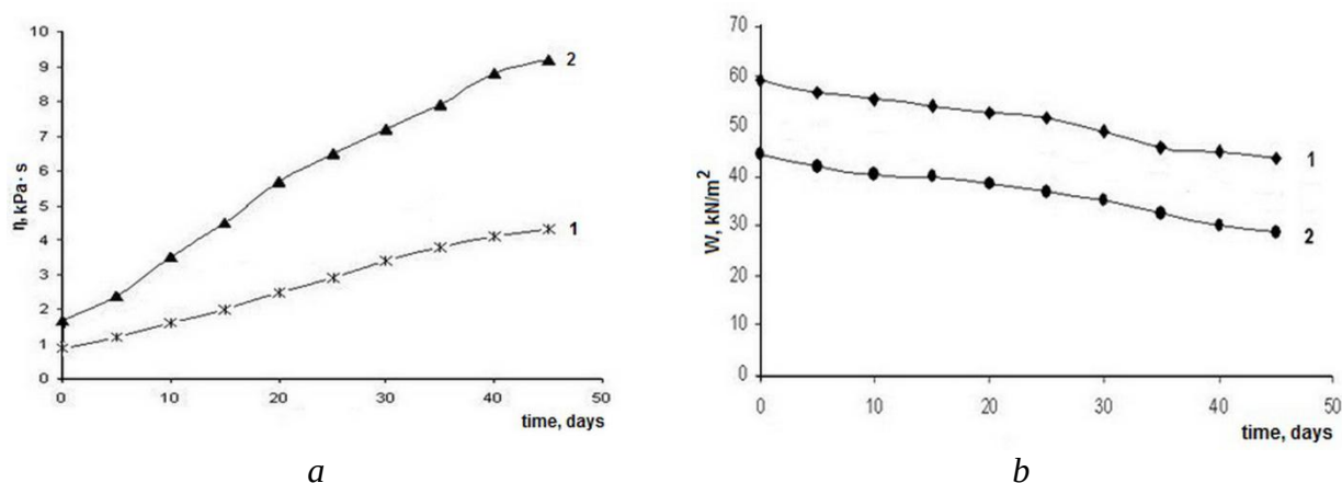
Fig. 1. Dynamic viscosity (a) and adhesive strength (b) vs. time of structure formation of PVA–CMC–STB polymer composites without fillers (1) and with silver sol (2)
