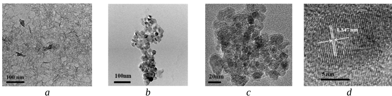
Fig. 1. HRTEM images of (a) \text{TiO}_2 , (b) VT1, (c) VT2 particles showing the morphology dispersed in sol prepared at the heating temperature of 95^\circ\text{C} for 12 h, and (d) HRTEM images of VT2 particles showing the lattice spacing of 0,347 nm corresponding to the anatase plane of (101)
