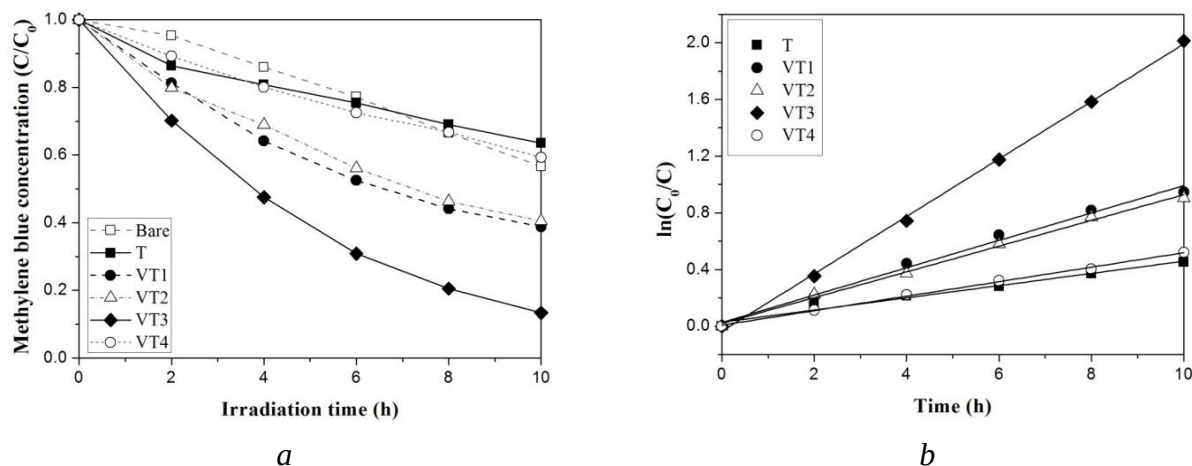
Fig. 3. Photocatalytic degradation of methylene blue under UV light irradiation by plotting (a) C/C_0 vs time (h) and (b) \ln(C_0/C) vs time (h)
